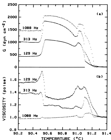
Figure 11. The elastic modulus and viscosity of CN at three different frequencies across the Isotropic (I)-N* transition showing three blue phases. Measuring device: torsional oscillators configured as cup viscometers with a cup diameter of 0.51 cm. Reproduced with permission from [44].
