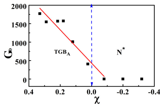
Figure 10. (Color online) Variation of G_0 with reduced temperature: \chi \equiv (T_{N^*-TGB_A} - T)/(T_{N^*-TGB_A}) . The solid line shows the best fit to G_0 \simeq \chi^\gamma , with \gamma = 1 . Reproduced with permission from [25].
